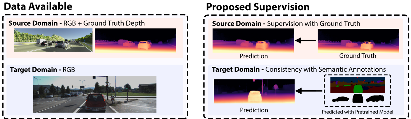
Fig. 1 Overview of the data available and proposed supervision. The source domain \mathcal{S} contains both RGB and ground truth depth data, and the target domain \mathcal{T} contains RGB data only. We train a depth estimation model to achieve high performance in \mathcal{T} by leveraging semantic annotations to introduce semantic consistency in \mathcal{T} . The semantic annotations are obtained using a panoptic segmentation model trained with external data.
