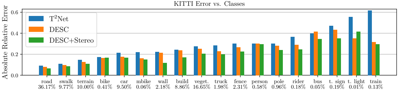
Fig. 7 Distribution of absolute relative error averaged over all pixels for a specific detected class over the KITTI Eigen test split (cap 80m) for models three different methods trained on Virtual KITTI→KITTI. The percentage of ground truth depth corresponding to each class is given below each class.
