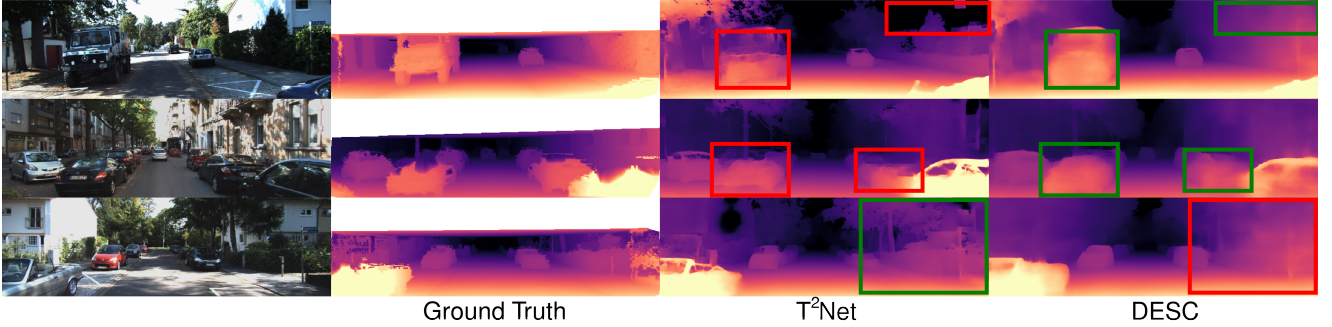
Fig. 3 Qualitative results in KITTI for models trained on Virtual KITTI→KITTI. Ground truth depth is linearly interpolated for visualization. Green bounding boxes refer to areas of the prediction more accurate compared to the corresponding red bounding boxes.
