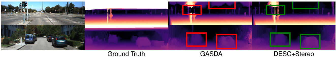
Fig. 5 Qualitative results in KITTI for models trained on Virtual KITTI→KITTI with stereo supervision in KITTI. Bottom row corresponds to a center crop of the original image.
