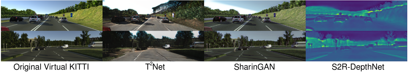
Fig. 8 Qualitative results for three different image transfer strategies. Virtual KITTI images are transferred to either a style matching KITTI images using a T 2 Net-based approach or to an intermediate shared domain with the transferred KITTI images using either a SharinGAN (PNVR et al., 2020) or S2R-DepthNet (Chen et al., 2021) approach. The original single-channel S2R-DepthNet images are mapped to RGB using a colormap and logarithmic mapping.
