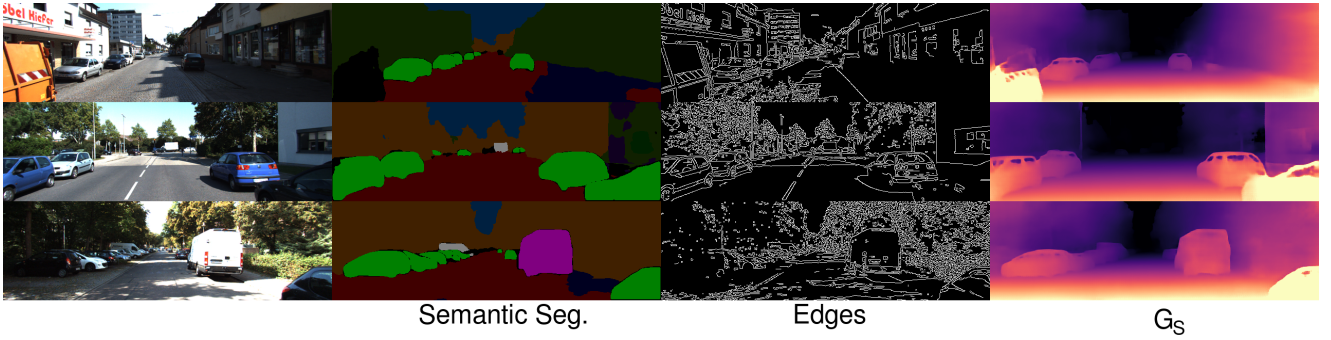
Fig. 4 Qualitative results of G_S , which takes as input the concatenation of the semantic and edge map.
