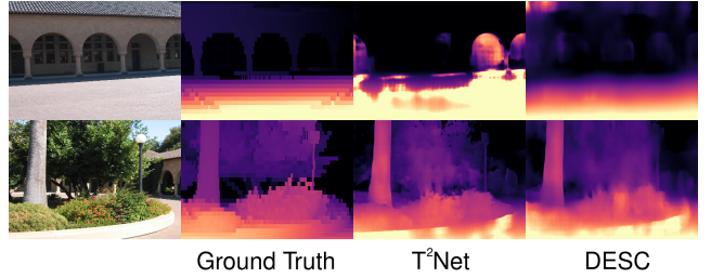
Fig. 10 Qualitative results in Make3D for T 2 Net and DESC.
