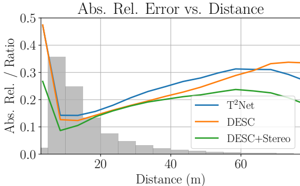
Fig. 6 Absolute relative error vs. ground truth distance for three different methods in the KITTI Eigen test split. We also include a histogram of the ground truth distribution. Left axis shows both absolute relative error (line plot) and ratio of ground truth values (histogram).
